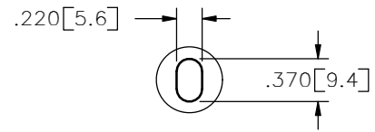
DETAIL A MOUNTING SLOTS TYP.
